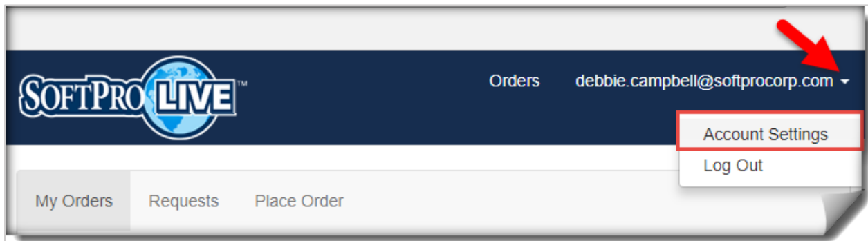
Figure 1.4: Account Settings
